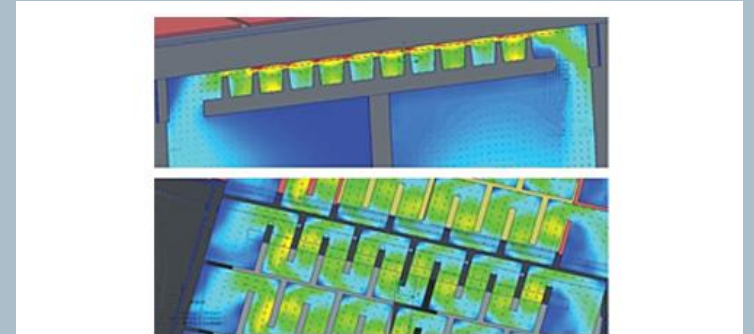
CFD simulation of power modules
