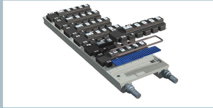
Danfoss ShowerPower® turbulators
